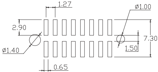
Recommended PCB Layout (PCB YDLERANCE±0.05)
